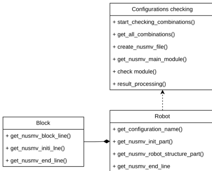
Figure 5.10: Class diagram of searching for relevant configurations
